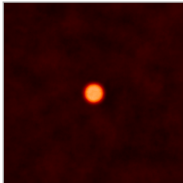
Tophat2DKernel
