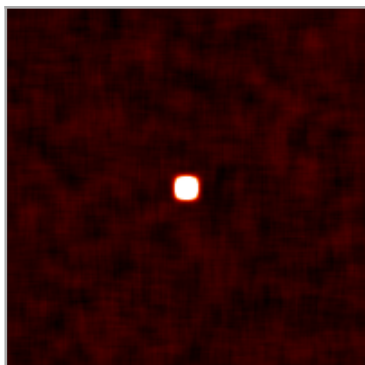
Box2DKernel
