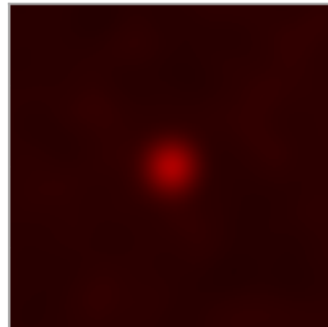
Gaussian2DKernel
