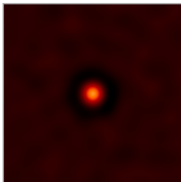
MexicanHat2DKernel
