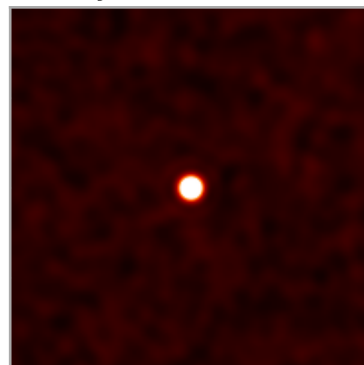
AiryDisk2DKernel
