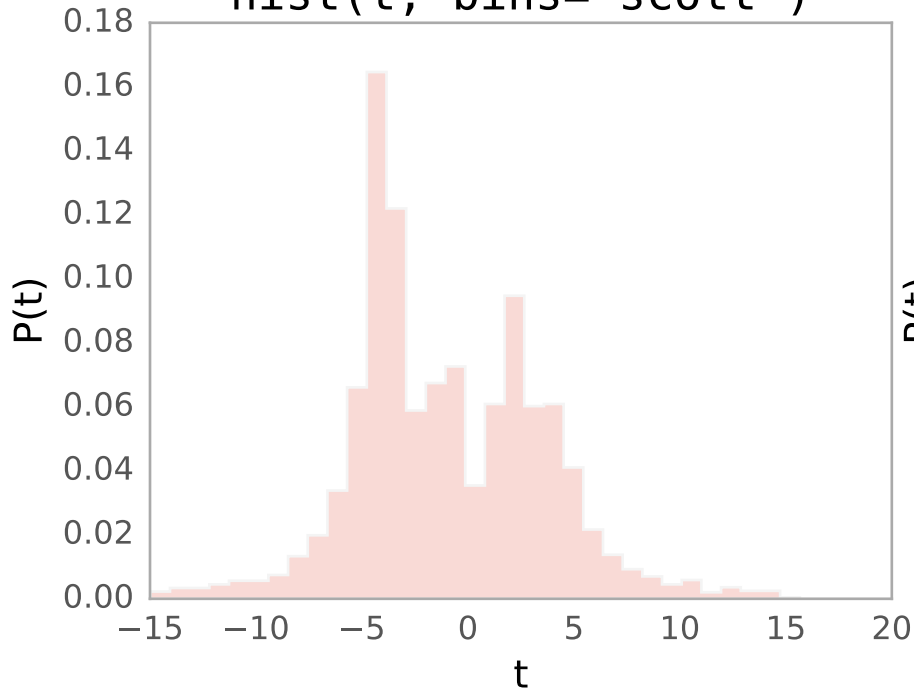
hist(t, bins="scott")
