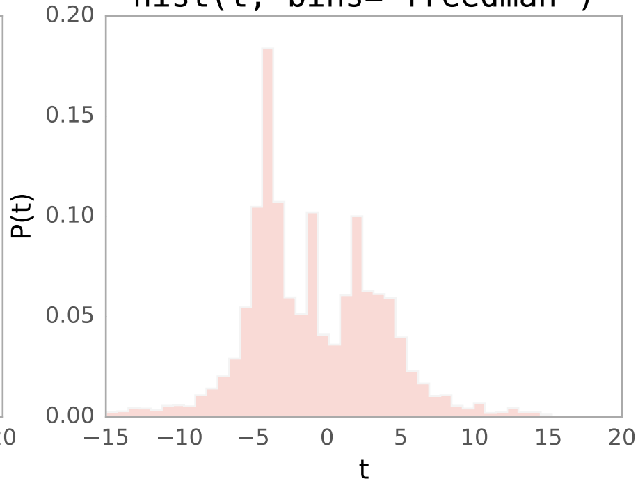
hist(t, bins="freedman")
