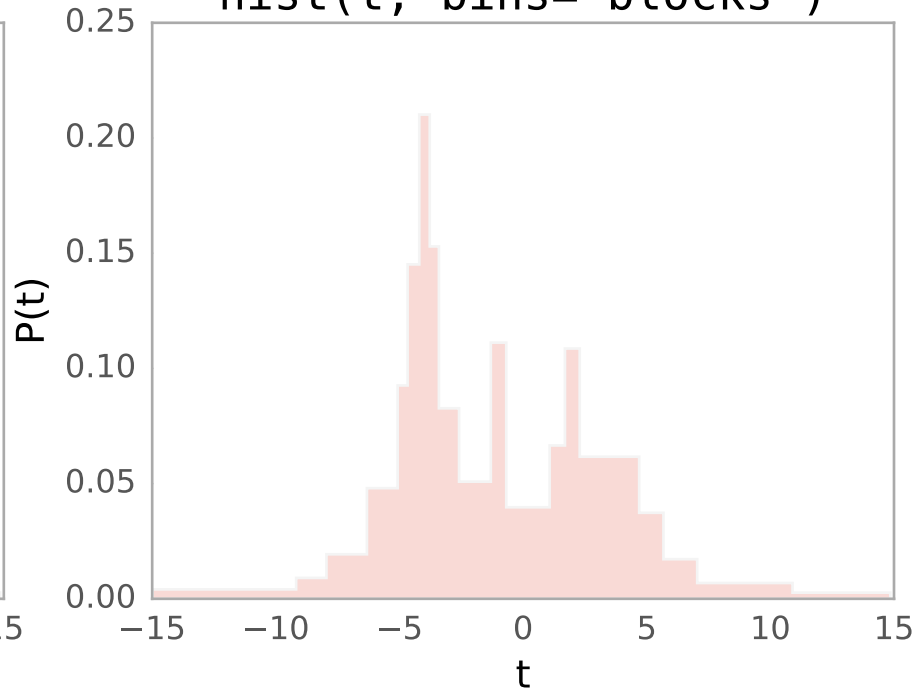
hist(t, bins="blocks")
