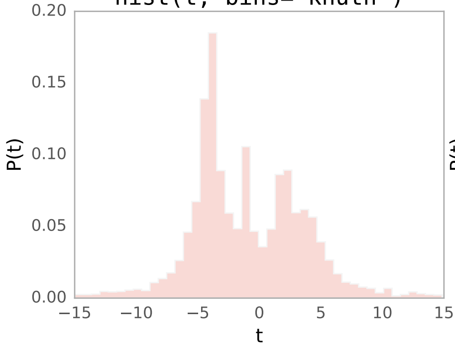
hist(t, bins="knuth")
